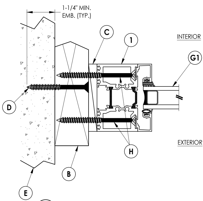
3 4 HORIZONTAL CROSS SECTION Shown w/ 2X Buck
