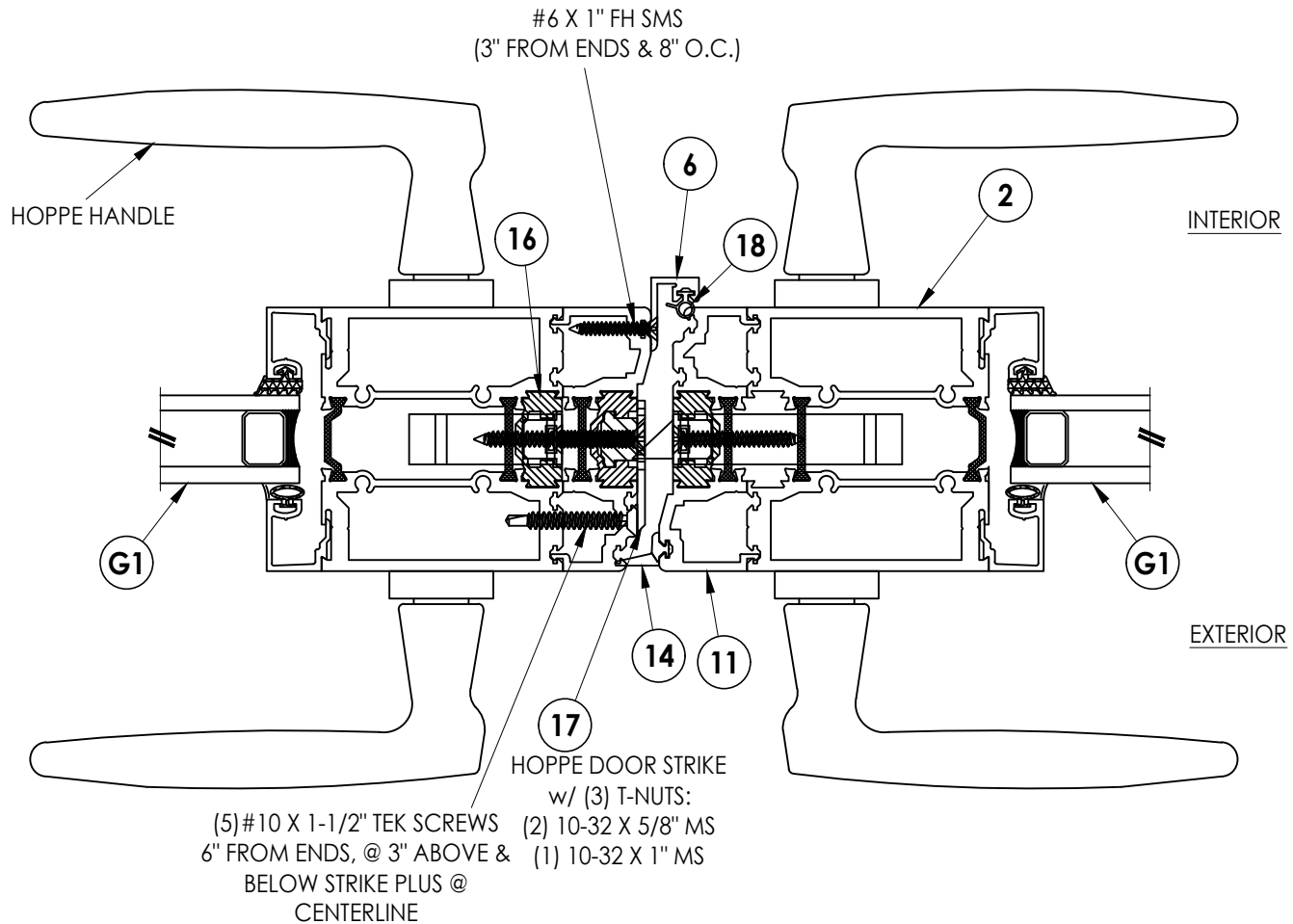
2 7 HORIZONTAL CROSS SECTION
