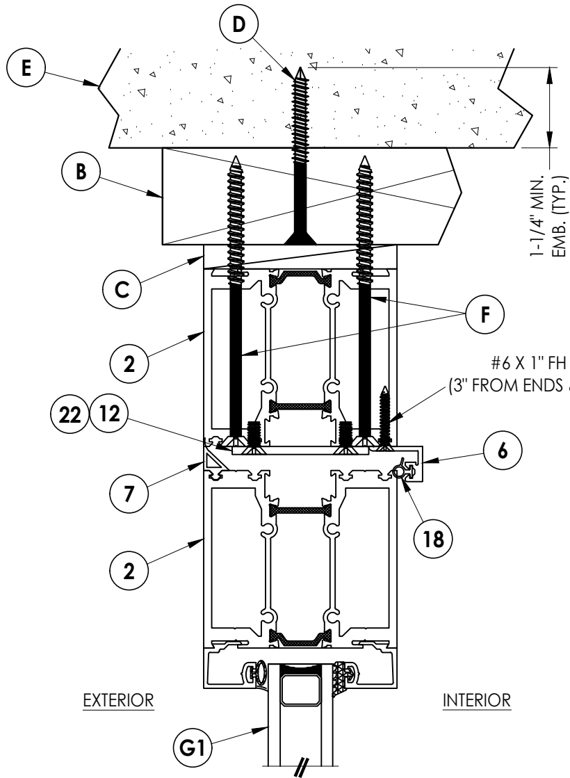
1 4 VERTICAL CROSS SECTION Shown w/ 2X Buck
